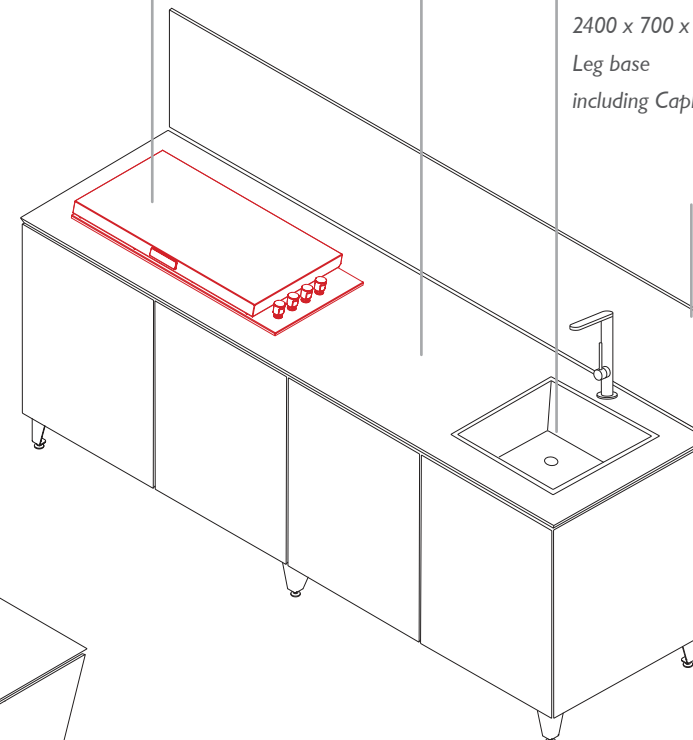
ADAPT 240 L 2400 x 700 x 900 Leg base
